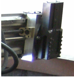
WP6000-9 Single point turning tool post, carriage, tools and drive
