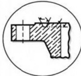
RTJ 'V' GROOVES
