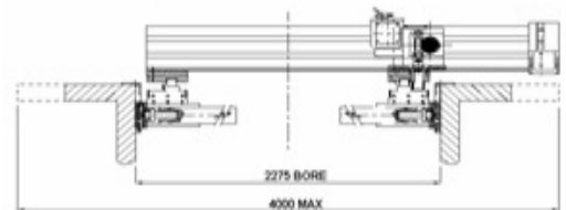
Internal mounting
