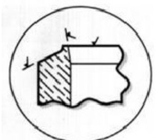
WELD PREPS
